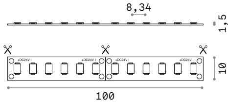
SMD 2835 120 LED/m
